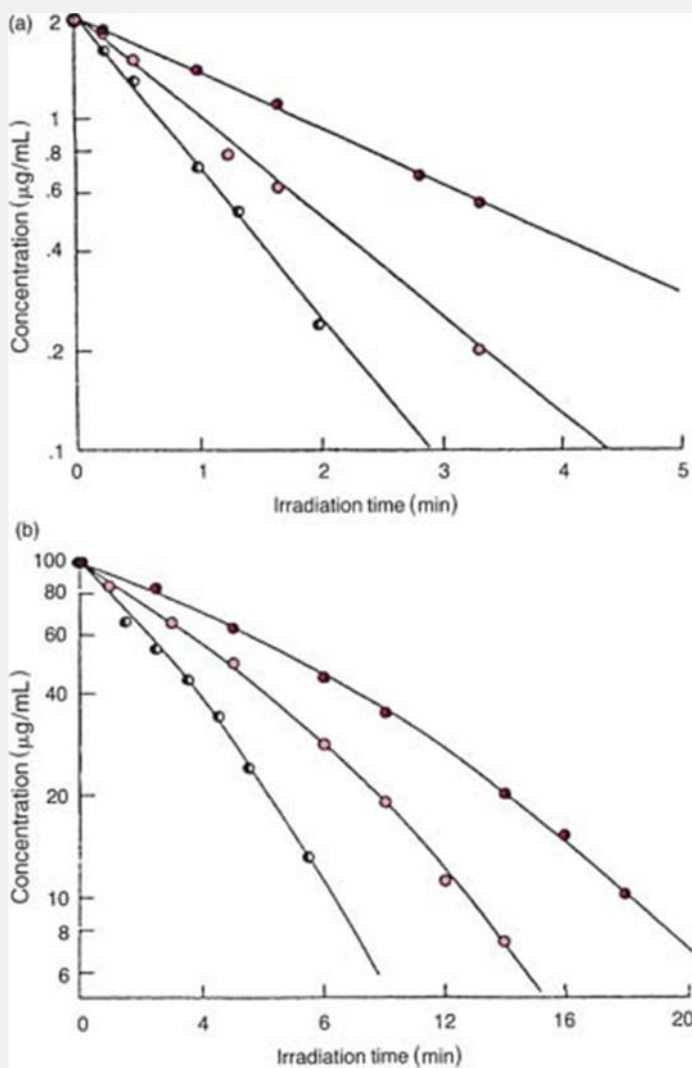
Fig. 14-18. A semilogarithmic plot of the photolysis of ketorolac tromethamine in ethyl alcohol. Key: \circ = under argon; \triangle = under air; \circ (with right half black) = under oxygen. (a) At low drug concentrations; (b) at high drug concentrations. (From L. Gu, H. Chiang, and D. Johnson, Int. J. Pharm. 41 , 109, 1988. With permission.)
